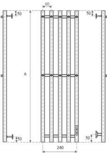
Blues Electro 100x27 П5 10 крючков MTRBLE10027
